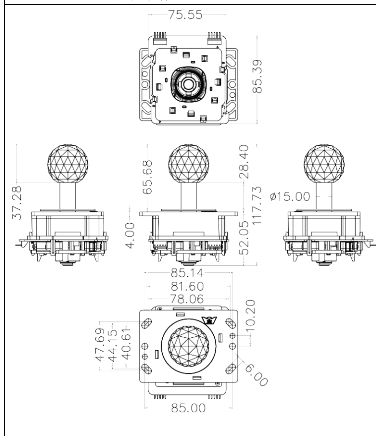
配短铁棒 With short shaft
