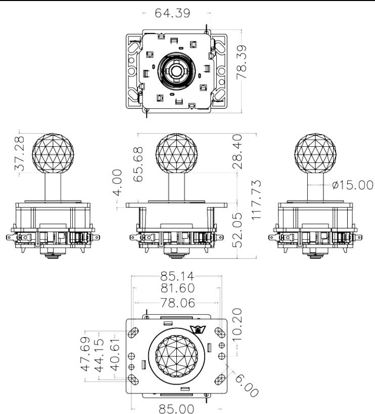
配短铁棒 With short shaft
